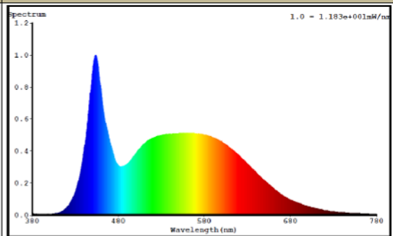
EBE-BSQ501-4.9W GU10 (6500K): 1#
