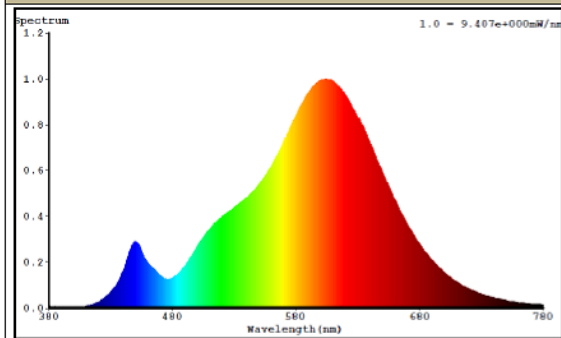
EBE-BSQ501-4.9W GU10 (2700K): 1#
