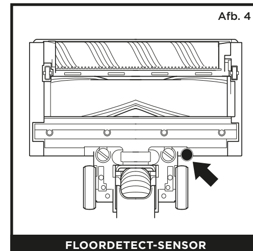
FLOORDETECT-SENSOR
